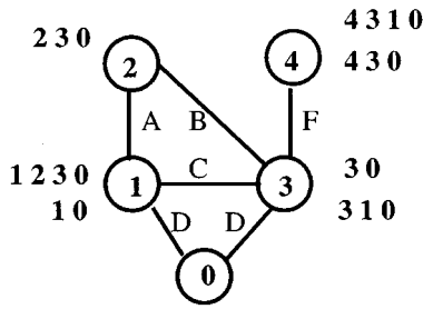
Fig. 12. The system INCOHERENT.
