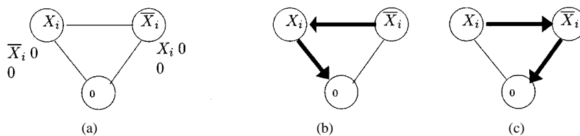
Fig. 7. Variable assignment gadget for X_i .
