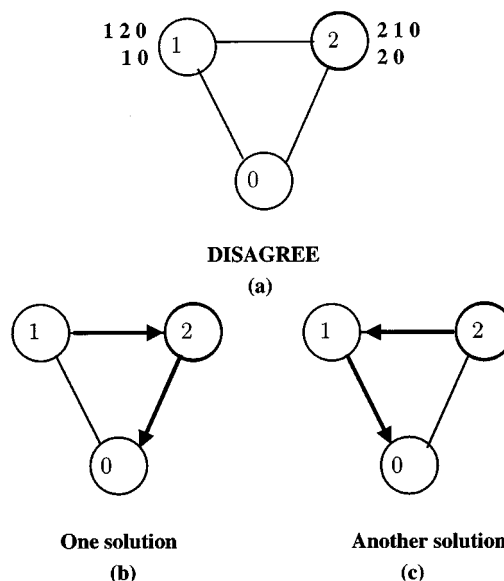
Fig. 3. DISAGREE and its two solutions.
