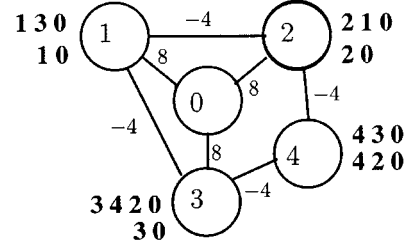
Fig. 11. NAUGHTY GADGET with negative link costs.
