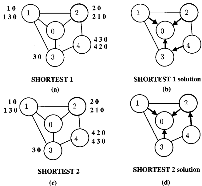
Fig. 1. Stable paths problems with shortest path solutions.
