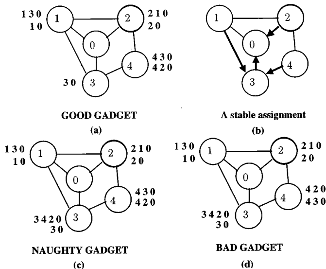
Fig. 2. Stable paths problems that are not shortest path problems.
