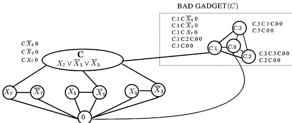
Fig. 8. Example of construction for clause C = X_7 \vee \bar{X}_5 \vee \bar{X}_3 .
