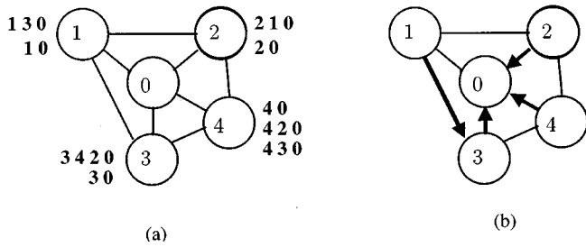
Fig. 4. (a) BAD BACKUP, a modification of BAD GADGET. (b) The unique solution.
