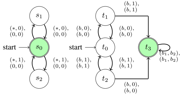
Figure 3. Automaton representing a function f_C which is non-zero outside the modified Cantor set. Note that we have two start states s_0 and t_0 . Each transition is labeled as (i, r), (i', r') where (i, r) represents the integer and fractional parts of the input; and (i', r') represents integer/fractional parts of the output. Here b denotes a 0 or 1 bit that has the same value in the input and output. We omit the transitions reading the sign of the input.
